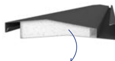
Louver Structure Sandwich construction with Peripor core
